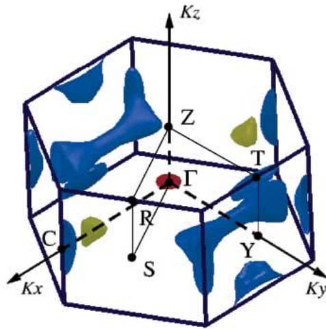
Fermi surface of solid metallic hydrogen at 414 GPa. The ab initio study predicts multiband superconductivity near room temperature. [P. Cudazzo, G. Profeta, A. Sanna, A. Floris, A. Continenza, S. Massidda, and E. K. Gross, Phys. Rev. Lett. 100 , 257001 (2008)]
